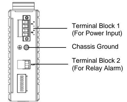
Figure 2. IPC-3014-PoE++ Media Converter Top Panel
