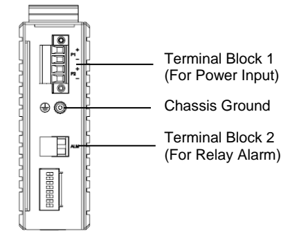
Figure 2. IPC-3012-PoE++ Media Converter Top Panel
