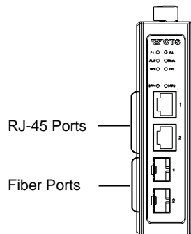
Figure 1. IAC-3014 Media Converter Front Panel
