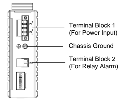
Figure 2. IAC-3012 Media Converter Top Panel
