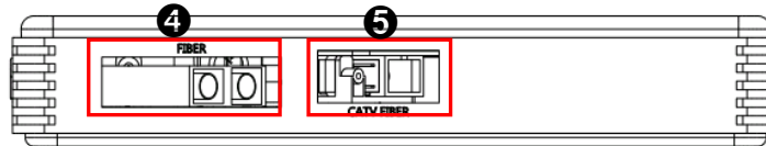
Figure 4. Rear Panel for 5 Ports 10/100/1000Base-T and 1 Port 1000Base-X or 100/1000Base-X Uplink Management Ethernet Switch with CATV RF Module
