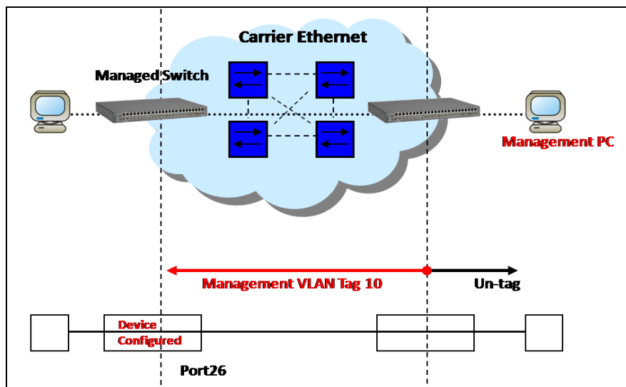
Management VLAN Network Diagram
