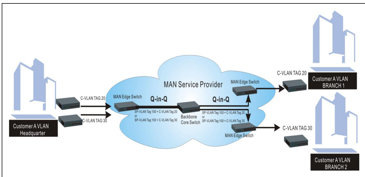
Q-in-Q Example
