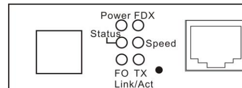
Figure 2. CVT-3002-PLUS WDM & SFP Front Panel
