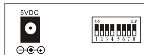
Figure 3. CVT-3002-PLUS Converter Rear Panel
