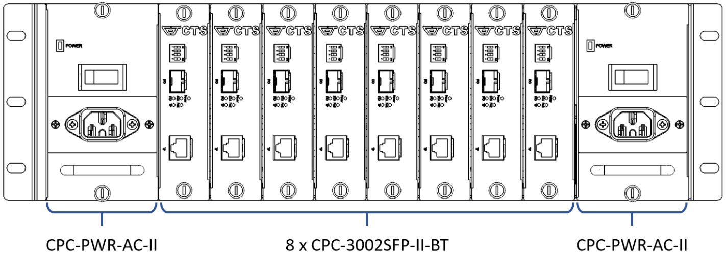
Figure 1. CPC-CHASSIS-08-II with 2 x CPC-PWR-AC-II and 8 x CPC-3002SFP-II-BT installed
